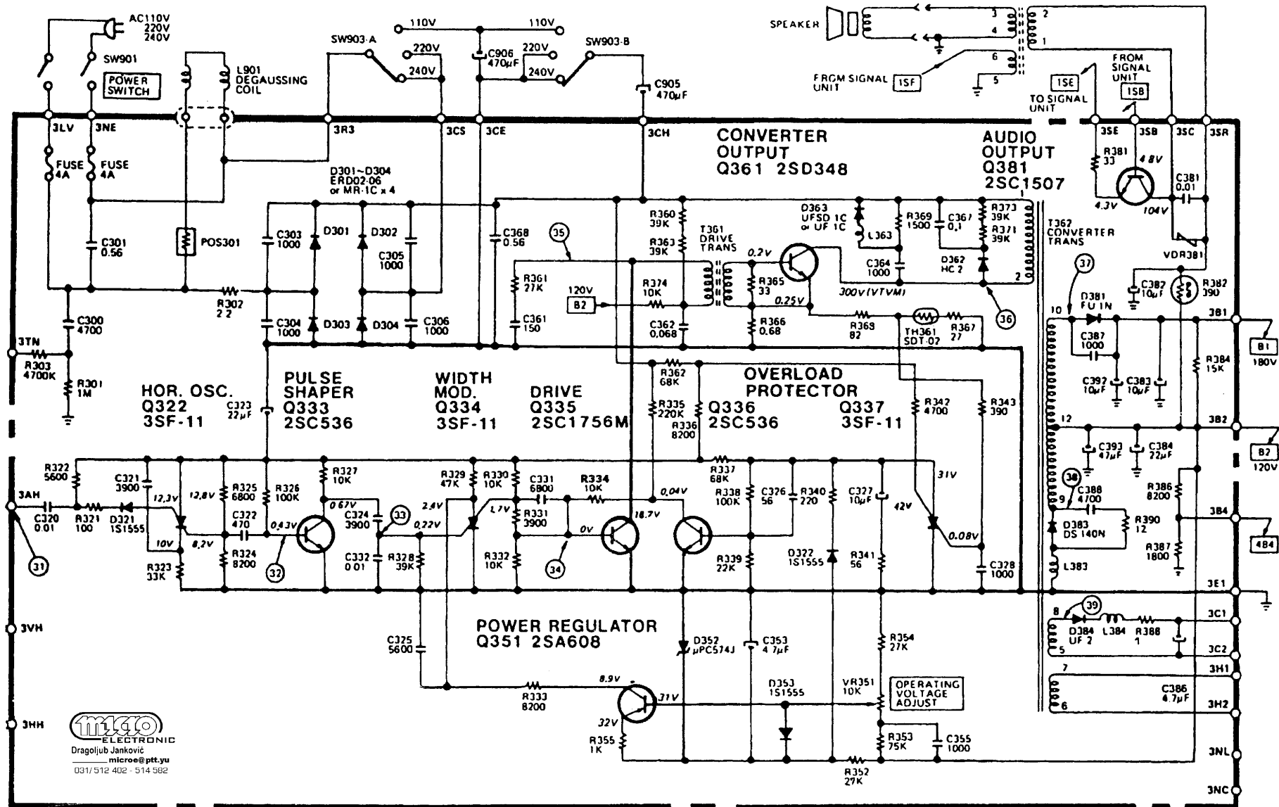
POWER-SUPPLY UNIT
