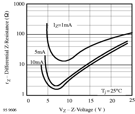
Figure 10. Differential Z-Resistance vs. Z-Voltage
