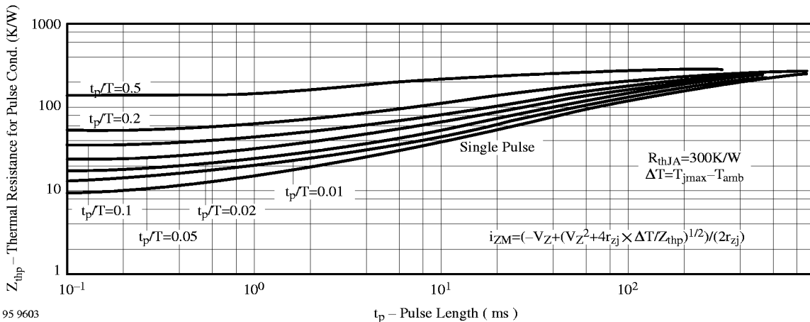
Figure 11. Thermal Response
