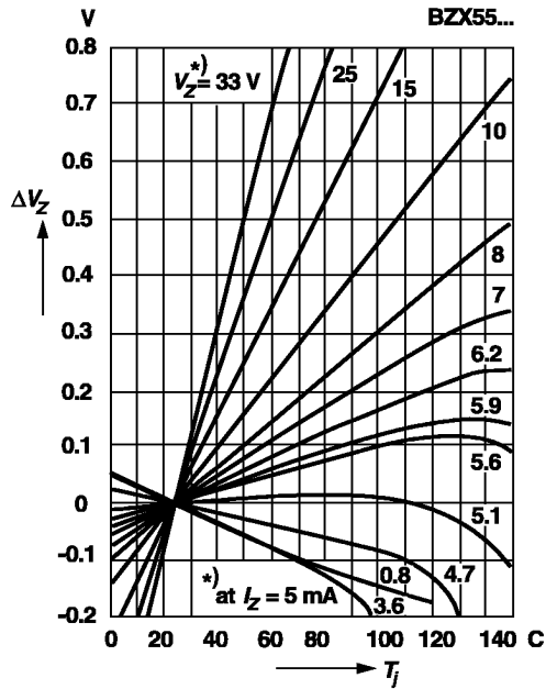
Change of Zener voltage versus junction temperature
