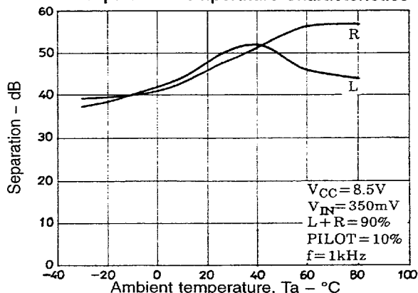
MPX Separation Temperature Characteristics
