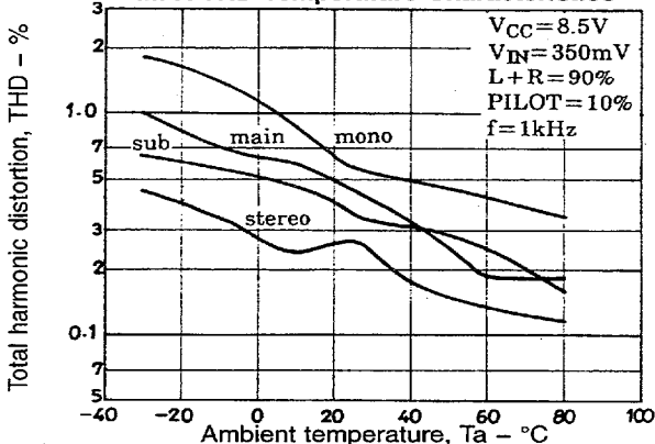
MPX THD Temperature Characteristics
