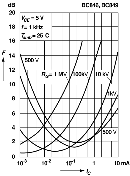
Noise figure versus collector current
