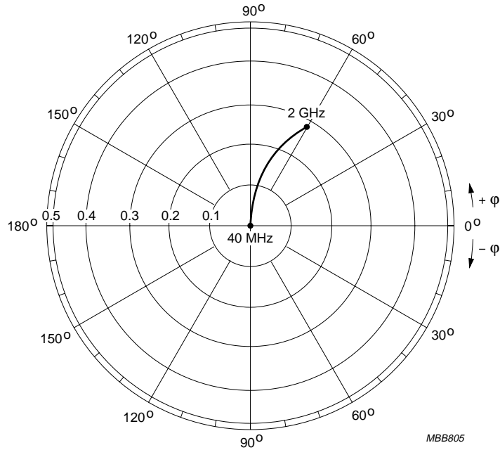
Fig.24 Common emitter reverse transmission coefficient ( S_{12} ).
