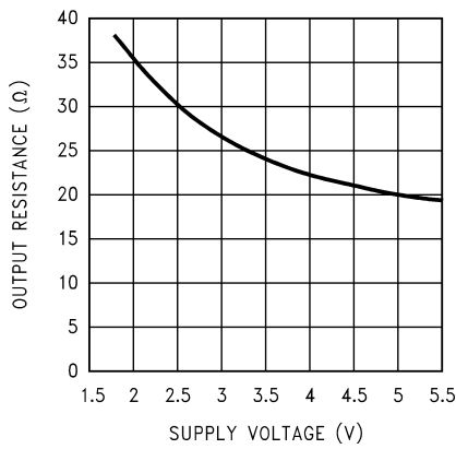
Output Resistance vs Supply Voltage
