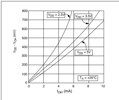
FIGURE 2-8: V_{DD} - V_{OH} vs. I_{OH}
